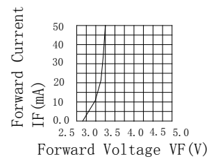
Fig 3. Forward Current vs. Forward Voltage
