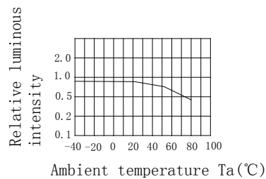
Fig 2. Relative Luminous Intensity vs. Ambient temperature (IF=20mA)
