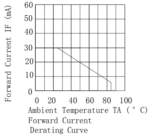
Derating Curve
