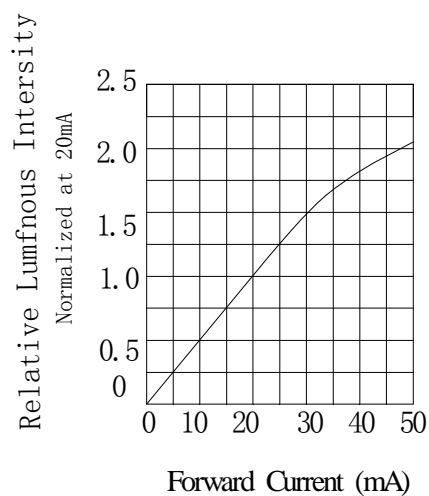
Fig.4 Relative Luminous Intensity vs. Forward Current
